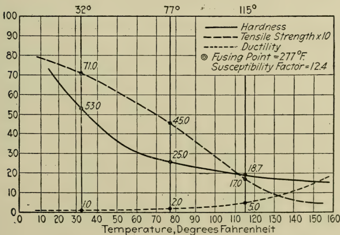
Fig. 53.—Chart of Physical Characteristics of Fluxed Oklahoma Grahamite Mixture.
